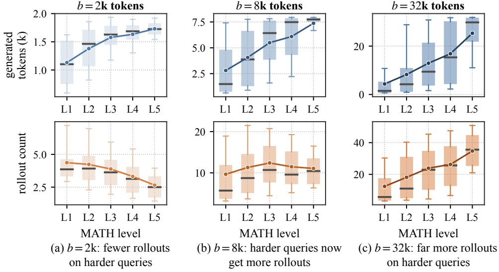
Figure 10: Allocation by MATH level on Llama-3.2-3B (PRICE-deployed with the self-evaluation score), with the same budgets and summaries as Figure 9. Token spending increases with difficulty at every budget, while the rollout count contrast between Level 1 and Level 5 reverses between 2k and 8k.
