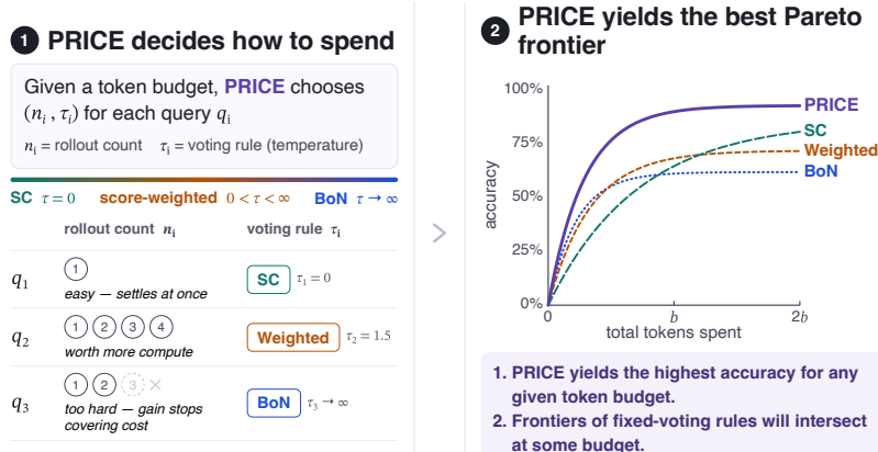
Figure 1: Illustration of the proposed PRICE method.
