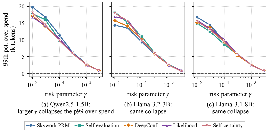
Figure 7: Empirical overspend relative to the risk budget ((a) Qwen2.5-1.5B, (b) Llama-3.2-3B, (c) Llama-3.1-8B; shared y range): p99 over-spend beyond b vs. \gamma at matched work ( \bar{n} \approx 8 per \gamma ), five scores. 99% of queries spend at most b plus the value shown; the dashed gray line marks zero over-spend, and the collapse is uniform across scores and generators.
