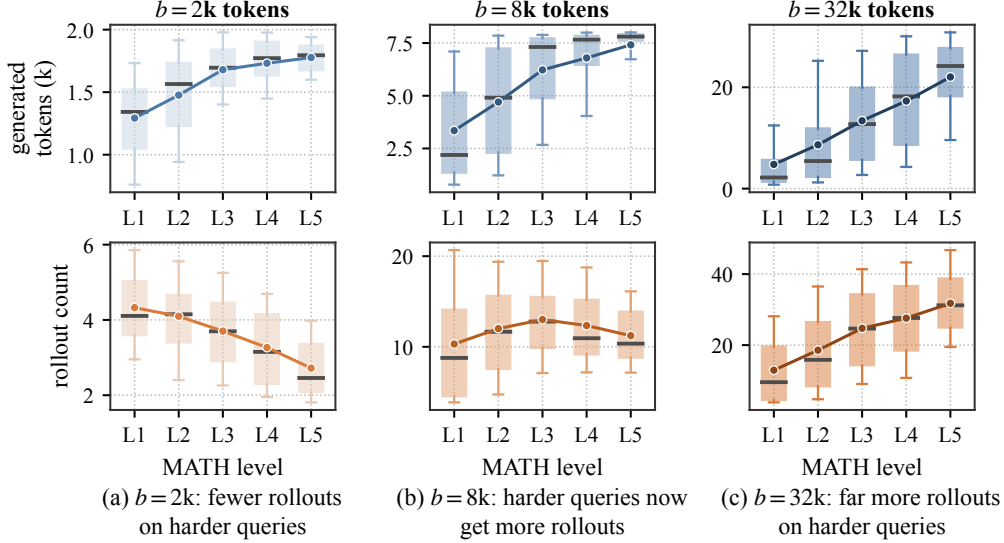
Figure 9: Allocation by MATH level of PRICE-deployed (Qwen2.5-1.5B; boxes = IQR with p10–p90 whiskers, dark-gray median, mean dot-line).
