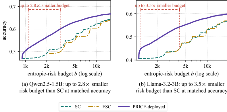
Figure 4: The frontier of PRICE-deployed against SC and ESC. The red dimension lines mark the accuracy at which the budget saving against SC is largest.
