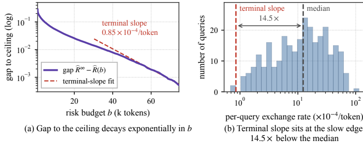
Figure 3: The large-budget law against the data (PRICE-oracle, Qwen2.5-1.5B).
