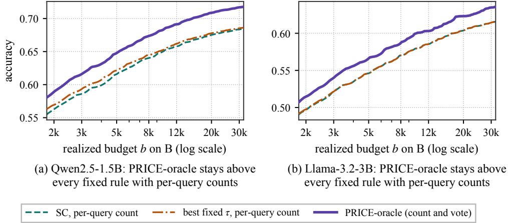
Figure 5: Split-pool frontiers of PRICE-oracle with the self-evaluation score ((a) Qwen2.5-1.5B, (b) Llama-3.2-3B). PRICE-oracle, the best global temperature and SC all choose per-query counts from the A primitives and are evaluated with the actual B token sums. The best global temperature is selected at each budget after seeing the results, so the orange curve is an envelope over fixed rules rather than a single policy.
