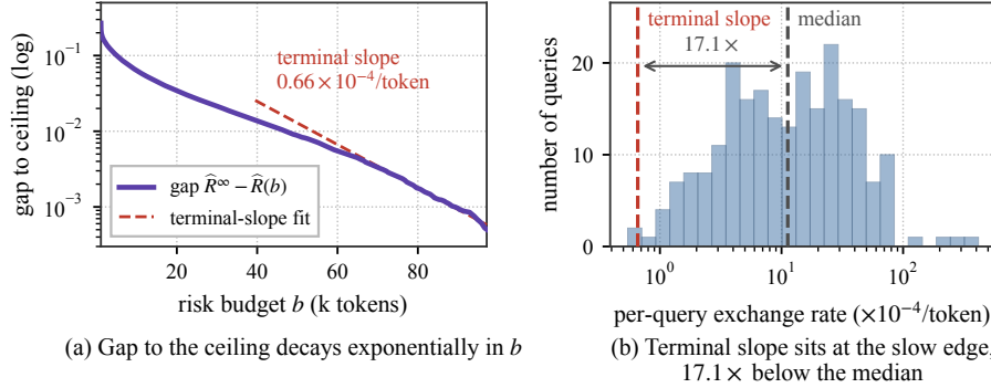
Figure 8: The large-budget law against the data on Llama-3.2-3B, with the protocol of Figure 3. The terminal slope is 0.66 \times 10^{-4} per risk-adjusted token, 17.1 \times below the median of the fitted exchange rates.
