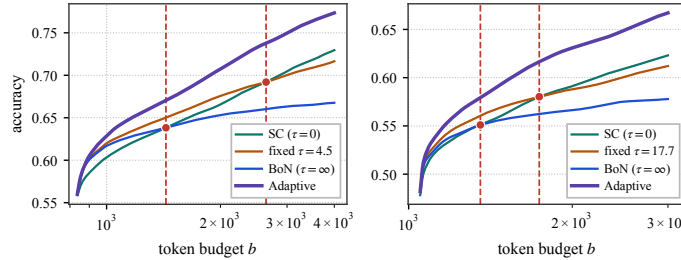
(a) Qwen2.5-1.5B: fixed rules swap the lead, adaptive on top (b) Llama-3.2-3B: same pattern
