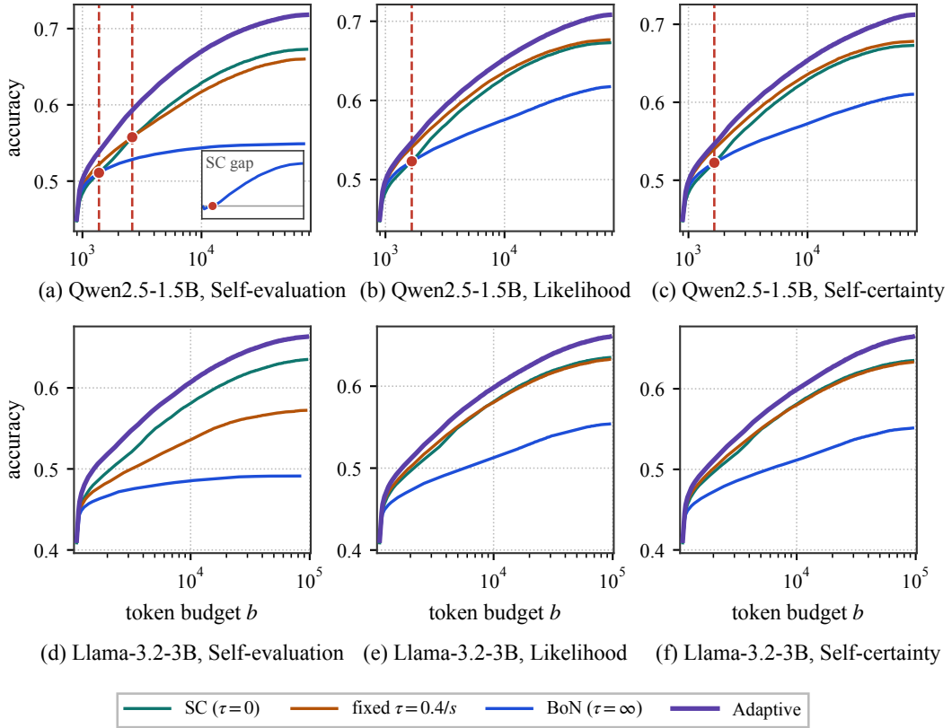
Figure 6: Figure 2 on the full MATH-500 population, with the Likelihood and Self-certainty scores added; panels (a)–(c) Qwen2.5-1.5B, (d)–(f) Llama-3.2-3B. Red dots mark the budgets at which the lead among the fixed rules swaps, and the inset in panel (a) shows the pairwise gap of SC over each competitor crossing zero. On the full Llama-3.2-3B population BoN leads SC only marginally at the smallest budgets, so panels (d)–(f) carry no markers.
